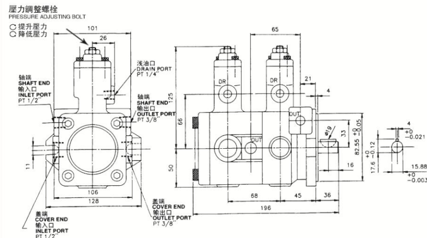
VP-F1212,F1515,F2020
